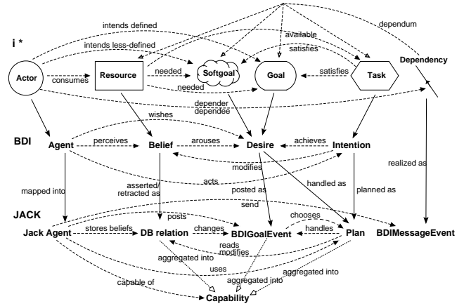
Figure 11: i*/BDI/JACK mapping overview
