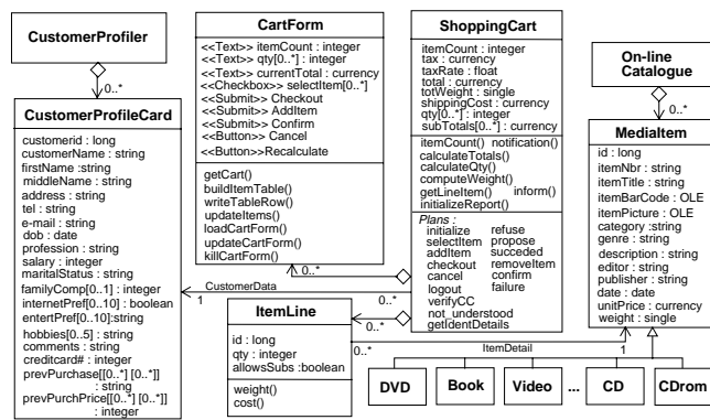
Figure 8: Partial class diagram for Store Front focusing on Shopping Cart
