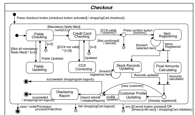
Figure 10: A plan diagram for checkout
