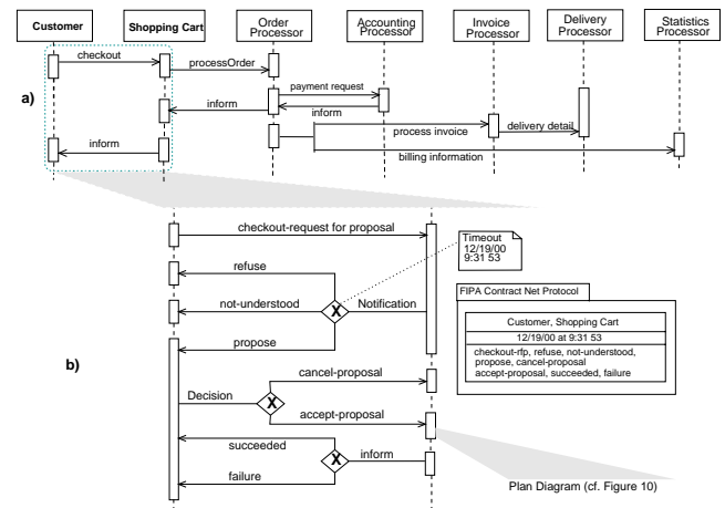
Figure 9: Sequence diagram to order media items (a), and agent interaction protocol focusing on a checkout dialogue (b)
