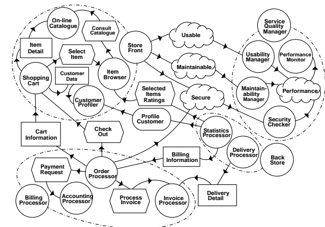
Figure 7: Strategic Dependency Model for Medi@ actors
