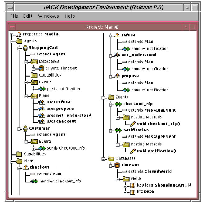
Figure 12: Partial implementation of Figure 9 in JACK
